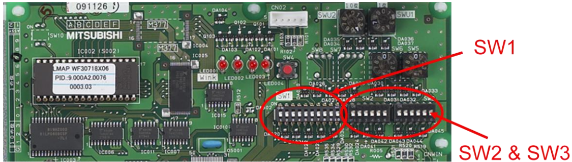
Figure 2. Dip Switch Locations on Control Board
